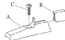
Lite Optic Front Sight Ref. 50611-LU
