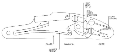
Internal Lock Parts Flintlock
