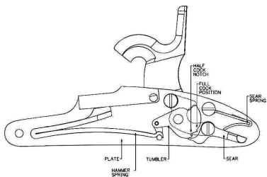
Internal Lock Parts Percussion
