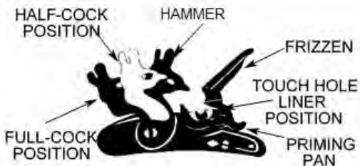
FLINTLOCK: EXTERNAL LOCK PARTS
